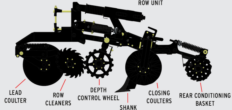
TERRAINPRO2 ROW UNIT
